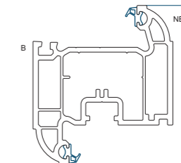
80mm Tilt & Turn Sash 103.267 Steel Reinforcement 113.373
