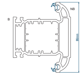
86mm T Mullion 102.263 Box Steel Reinforcement 113.041 U Channel Steel Reinforcement 113.321 C Steel Reinforcement 113.378 Cranked Steel Reinforcement 113.371 Ported Aluminium Reinforcement 115.285
