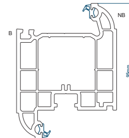
95mm Z Double Door Sash 103.265 U Channel Steel Reinforcement 113.375 Prepared U Channel Steel Reinforcement 113.374
