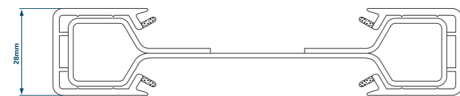
Dog Bone Coupling 113.112 Cover 116.012
