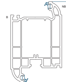
110mm Z Residential Door Sash 105.168 Box Steel Reinforcement 113.231 U Channel Steel Reinforcement 113.320 Prepared U Channel Steel Reinforcement 113.318
