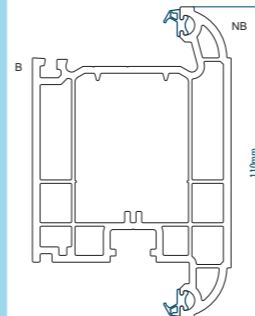
110mm T Residential Door Sash 105.169 Box Steel Reinforcement 113.231 U Channel Steel Reinforcement 113.320 Prepared U Channel Steel Reinforcement 113.318
