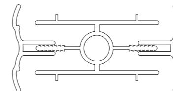
25mm Loadbearing 10148
