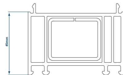
45mm frame extension 114.202 Reinforcement 113.271
