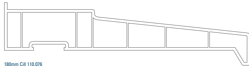
180mm Cill 110.076
