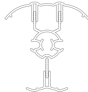
Loadbearing Variable Pole 10145
