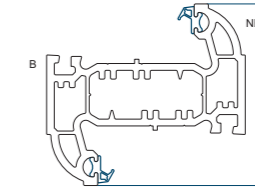
64mm Z Mullion 102.260 Box Steel Reinforcement 113.041 U Channel Steel Reinforcement 113.321 Ported Aluminium Reinforcement 115.284
