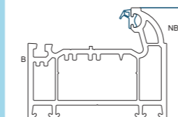
56mm Outer Frame 101.160 Steel U Channel Reinforcement 113.317
